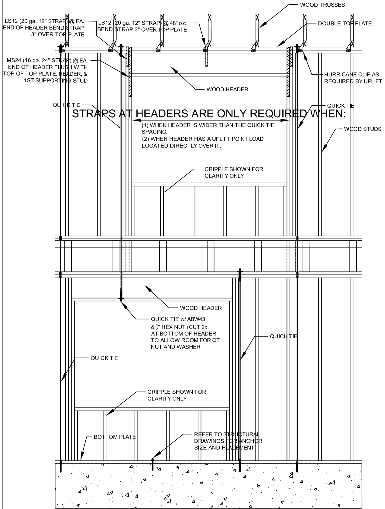
TYPICAL OFFSET HEADER TIE DOWN DETAILS
