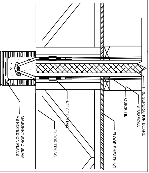
MASONRY/WOOD FIRE SEPERATION WALL QUICK TIE INST. DETAIL
