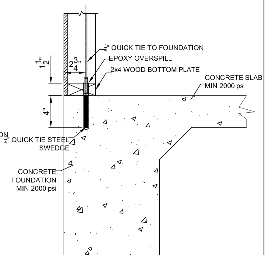
MONOLITHIC SLAB QUICK TIE INSTALLATION DETAIL
