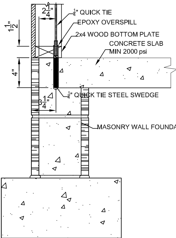
STEM WALL QUICK TIE INSTALLATION DETAIL
